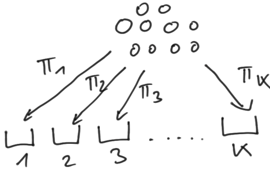
Figure 5.1: Multinomial urn model.
