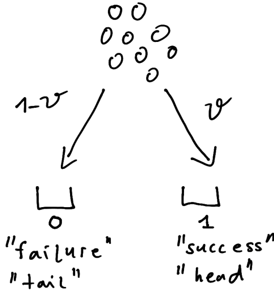
Figure 4.1: Binomial urn model.
